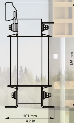
Figure 3: Transformer lateral side
